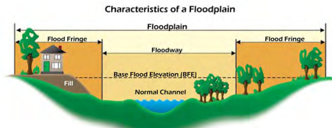
Figure 4 Characteristics of a Floodplain
