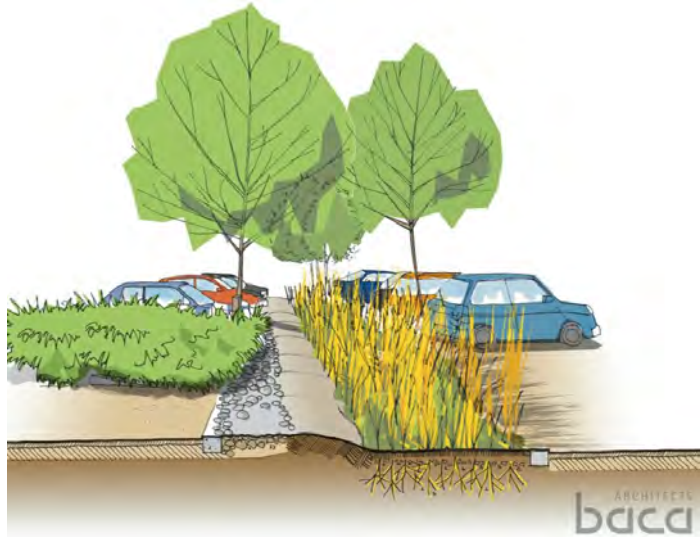
Figure 15 Vegetated Filter Strip
